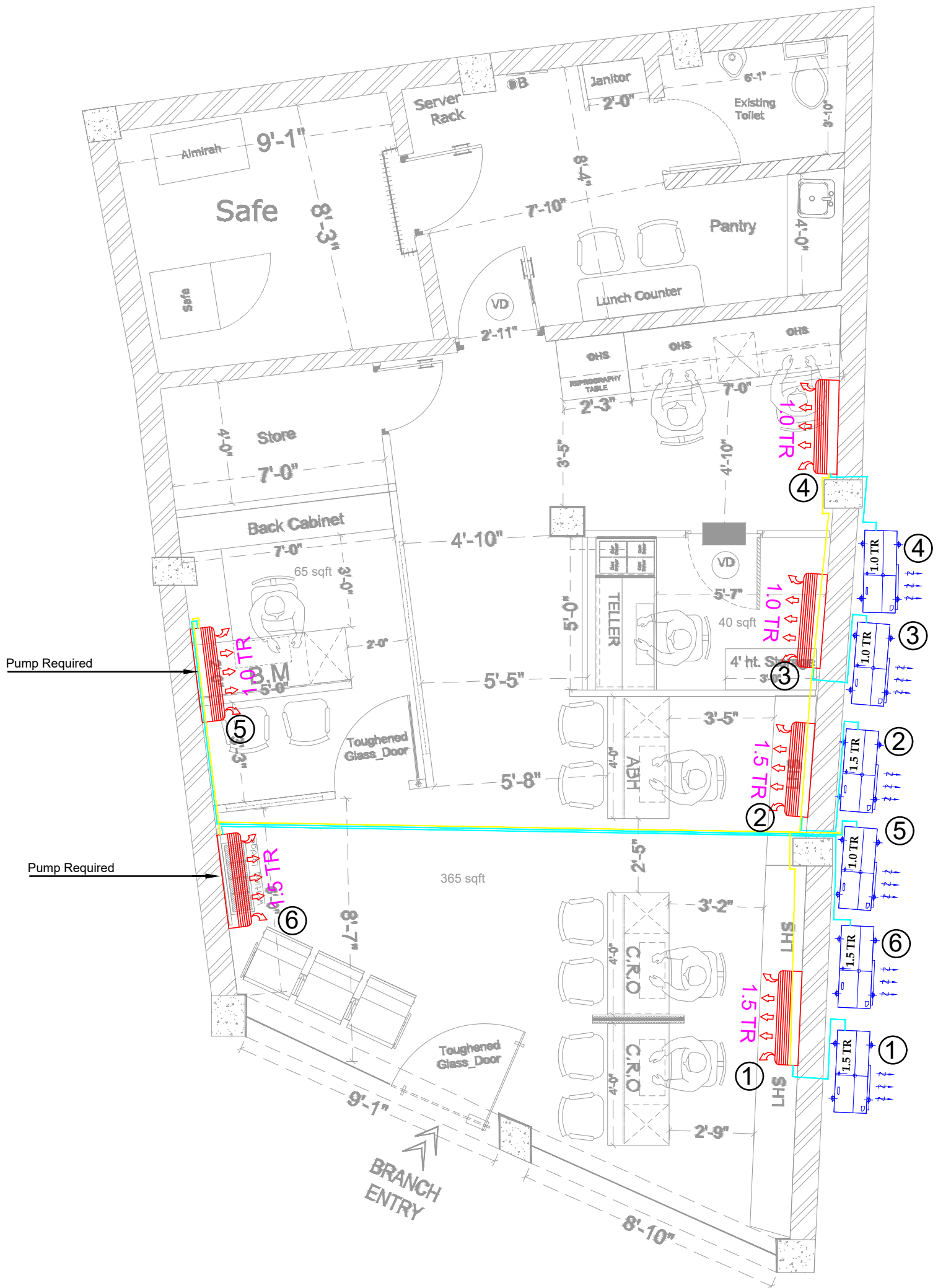
LAKHIPUR BRANCH GROUND FLOOR
