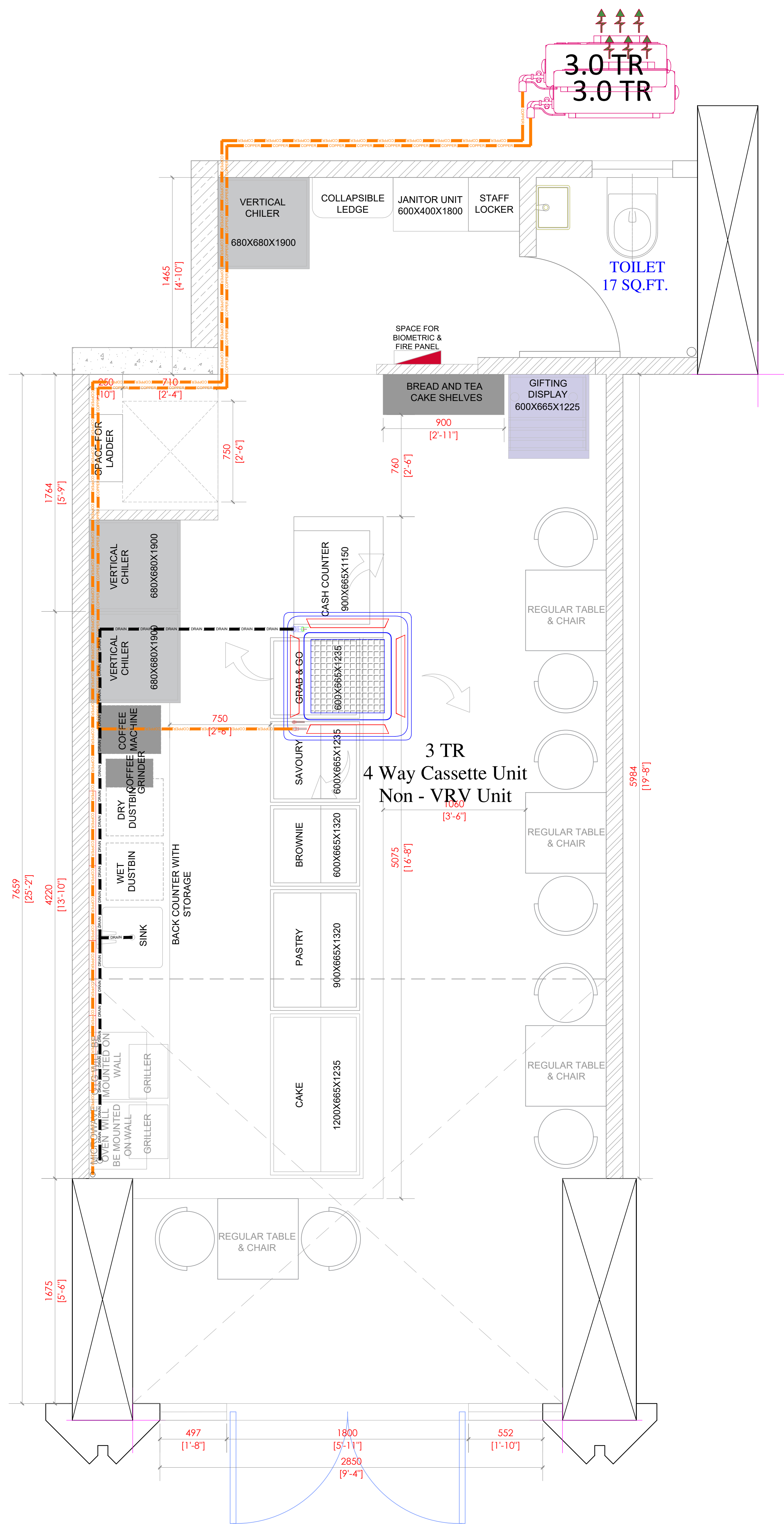
GROUND FLOOR PLAN TOTAL AREA : 345 SQ.FT NO OF SEATING : 6 NOS.
