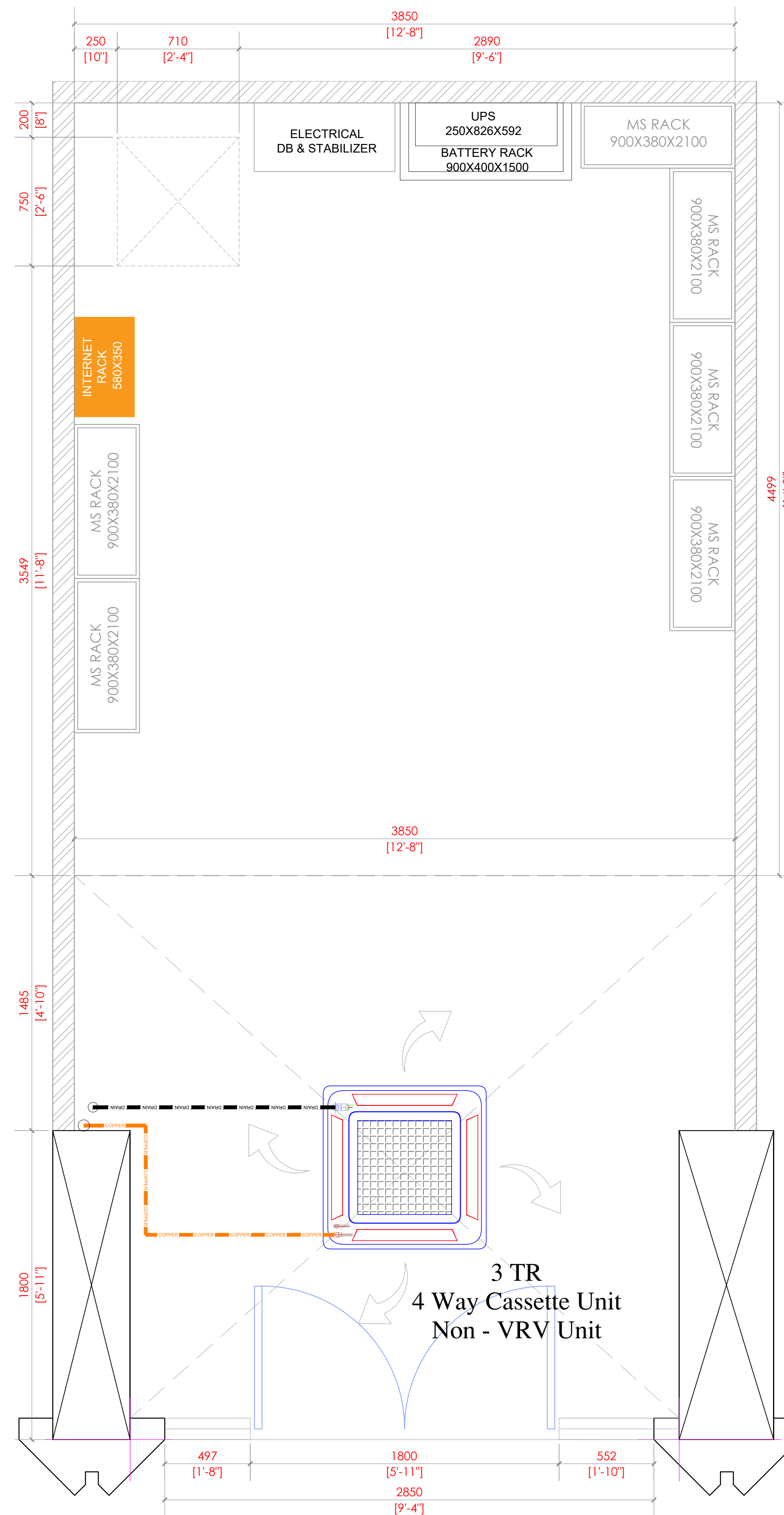
MEZZANINE FLOOR PLAN TOTAL AREA : 181 SQ.FT NO OF SEATING : 0 NOS.
