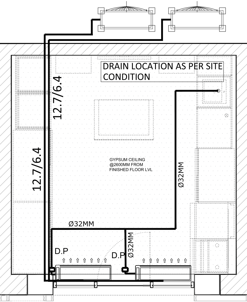
HVAC LAYOUT 1:35 H-301
