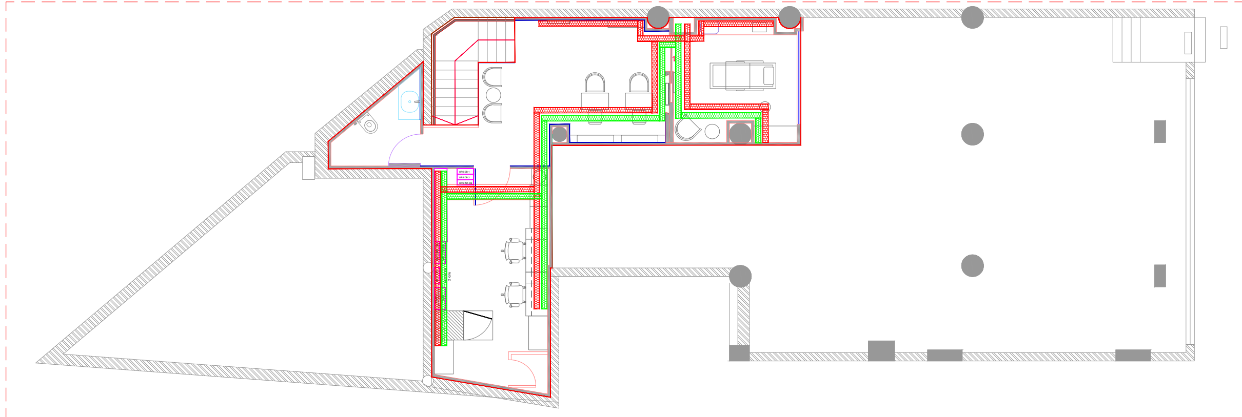
POWER SOCKET & DATA/VOICE LAYOUT Scale: 1 : 75
